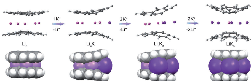
Figure 4. Transformation of alkali-metal cores starting from \text{Li}_5 to \text{LiK}_5 sandwiches. Some intermediates are omitted.
